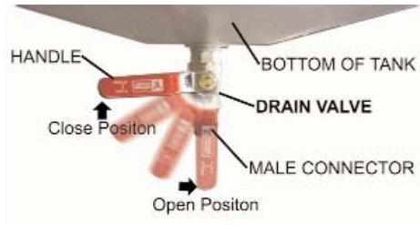
Drain Valve
